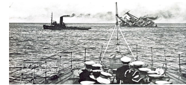
HMAS AUSTRALIA I - SCUTTLED AND SINKING - 1924 - WASHINGTON NAVAL TREATY
